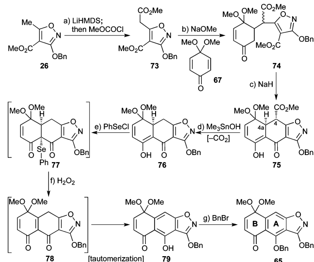
Scheme 9. First Synthesis of AB-Quinone Monoketal 65 a
