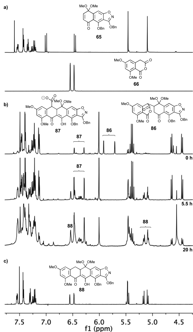
Figure 2. Monitoring the coupling of cyclic anhydride 66 and AB-quinone monoketal 65 by ^1\text{H} NMR spectroscopy (MeCN- d_3 , 500 MHz): (a) ^1\text{H} NMR spectra of starting materials 65 and 66 ; (b) ^1\text{H} NMR spectra during reaction (0, 5.5, and 20 h); (c) ^1\text{H} NMR spectrum of product 88 after purification.
