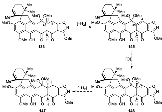
Scheme 26. Attempted Preparation of Olefin 145 a
