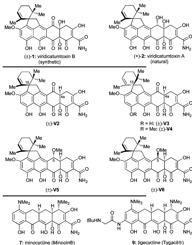
Chart 3. Molecular Structures of Natural Viridicatumtoxin A ( 2 ), Synthetic Viridicatumtoxin B ( 1 ), Synthesized Viridicatumtoxin Analogues ( V2–V6 ), and Tetracycline Drugs Minocycline ( 7 ) and Tigecycline ( 9 )
