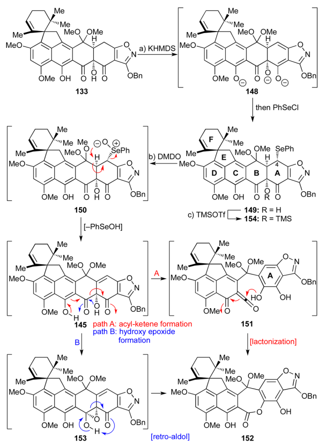
Scheme 26. Attempted Preparation of Olefin 145 a
