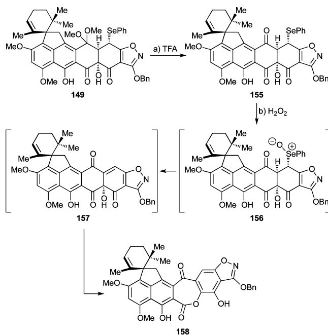
Scheme 27. Attempted Preparation of Enone 157 a
